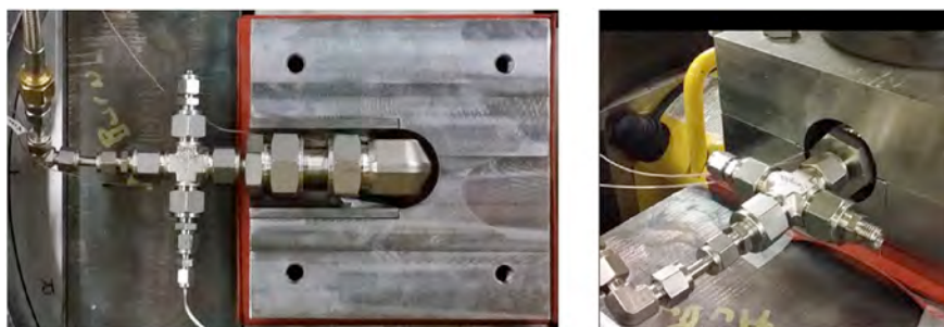
Fig. 7. Setup for coaxial cryogen flow through – for confined specimen tests.
