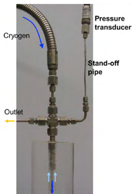
Fig. 10. Stand-off pipe placed vertically to support measurements of borehole pressure.
