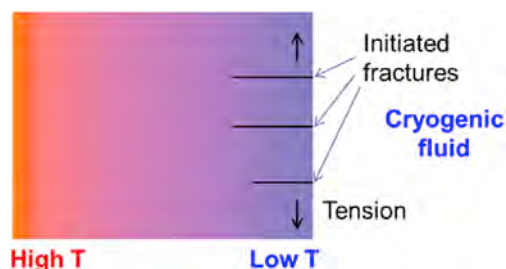
Fig. 1. The basic concept of cryogenic fracturing.
