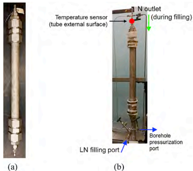
Fig. 4. Liquid nitrogen transfer cylinder for higher-pressure LN flow. (a) 5.1 cm-OD stainless steel tubing. (b) Assembled to the system. (Photo taken before applying insulation).
