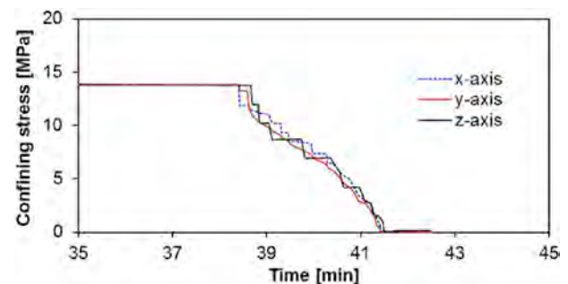
Fig. 16. An example of synchronized unloading to avoid large stress anisotropy, using pressure relief valves in the hydraulic system.
