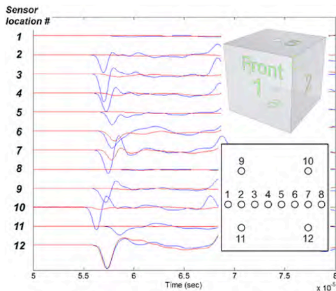
Fig. 20. An example of P-wave signatures before (blue lines) and after (red lines) liquid nitrogen treatment in a concrete specimen (wave transmission between Faces 1&3). (For interpretation of the references to colour in this figure legend, the reader is referred to the web version of this article.)
