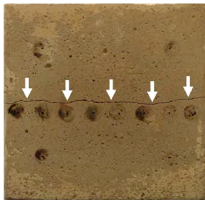
Fig. 15. Prominent fracture along the centers at the sides in a concrete specimen created due to repeated, acute anisotropic conditions (sudden unloading of z-axis only).
