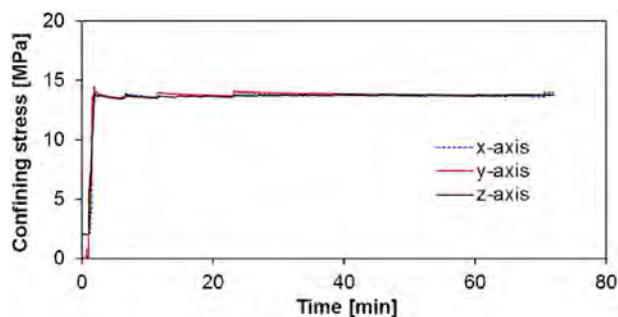
Fig. 14. Confining load tests – manual control of constant stress (isotropic 14 MPa).
