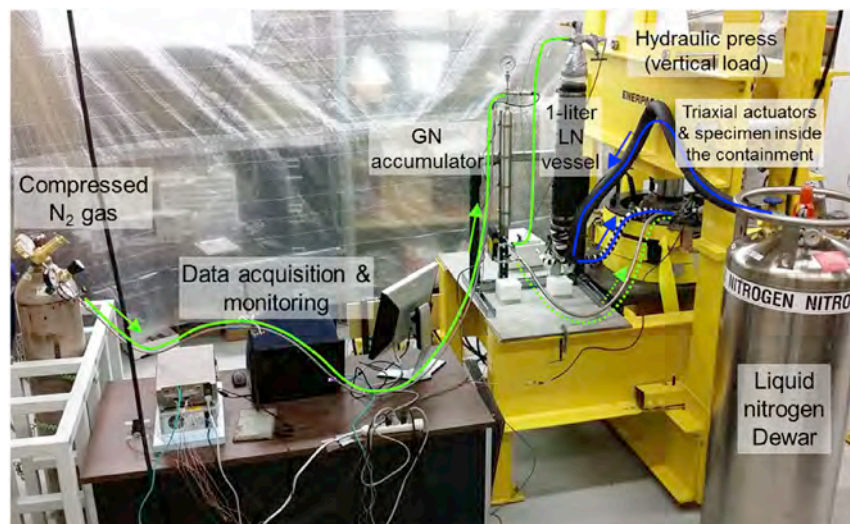
Fig. 13. Assembled setup for cryogenic stimulation tests under specimen confining load. Green lines are tubes for pressurized gas nitrogen and blue lines are for tubes for liquid nitrogen. (For interpretation of the references to colour in this figure legend, the reader is referred to the web version of this article.)
