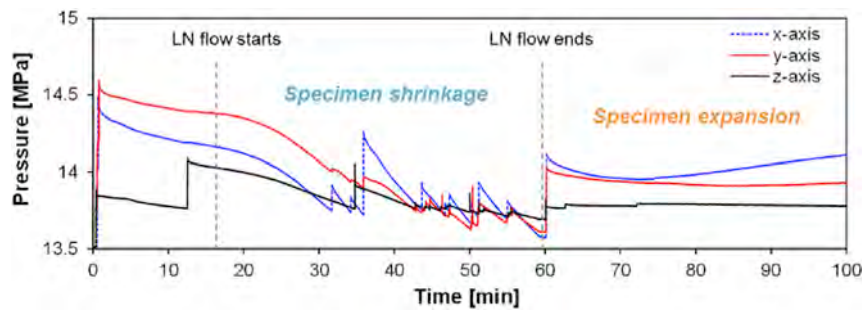
Fig. 18. Shrinkage and expansion of a concrete specimen due to specimen cooling and warming, indicated from hydraulic pressure responses during low-pressure LN flow (followed by pressurization).
