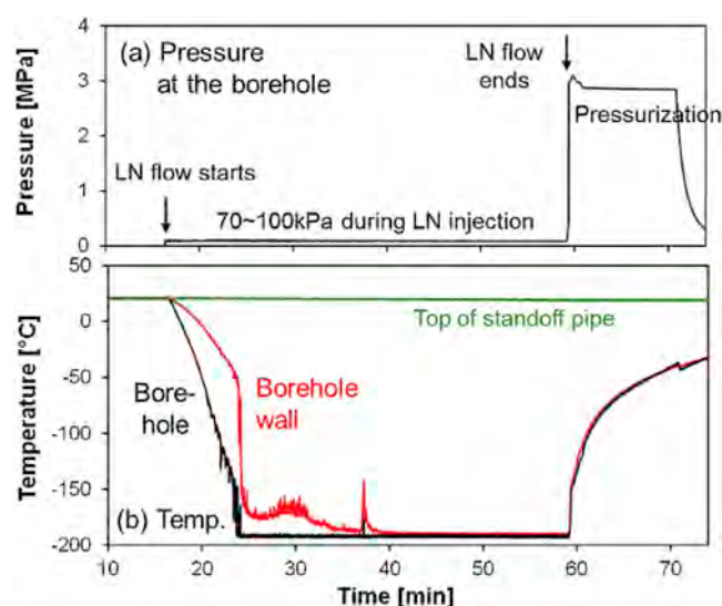
Fig. 17. Borehole pressure and temperature during low-pressure LN flow followed by borehole pressurization in a concrete specimen under 14 MPa isotropic confining stress.
