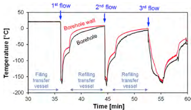
Fig. 19. Temperature changes during multiple higher-pressure LN flow-through.
