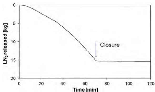
Fig. 11. Typical liquid nitrogen consumption vs. time.
