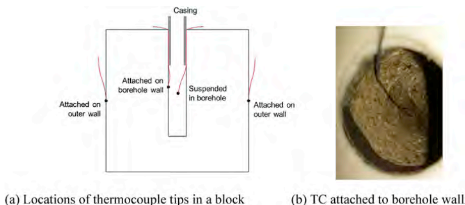
Fig. 8. Thermocouple instrumentation on a test block.
