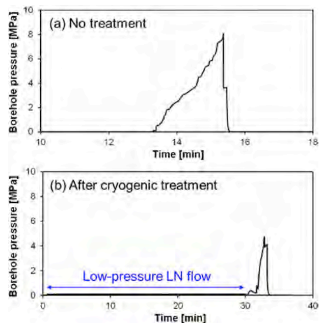
Fig. 21. Post-stimulation breakdown fracturing of a concrete specimen by nitrogen gas pressure.
