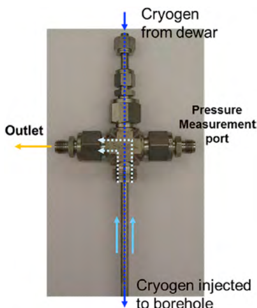
Fig. 6. Coaxial design for cryogen flow through the borehole – for unconfined specimen tests (the casing detached to show the inner inlet pipe).
