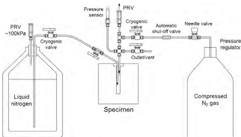
Fig. 2. Basic schematic of lab cryogenic stimulation setup under low-pressure LN flow (the triaxial loading device not shown). Compressed nitrogen gas can be used to pressurize boreholes.
