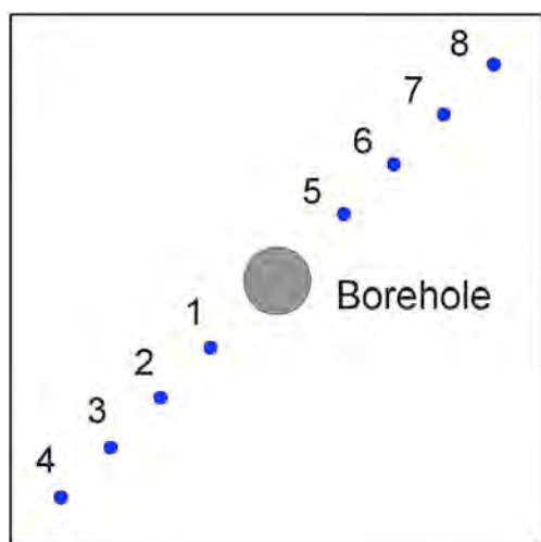
Fig. 9. Locations of TC tips inside a concrete block at its mid-height for temperature measurements.
