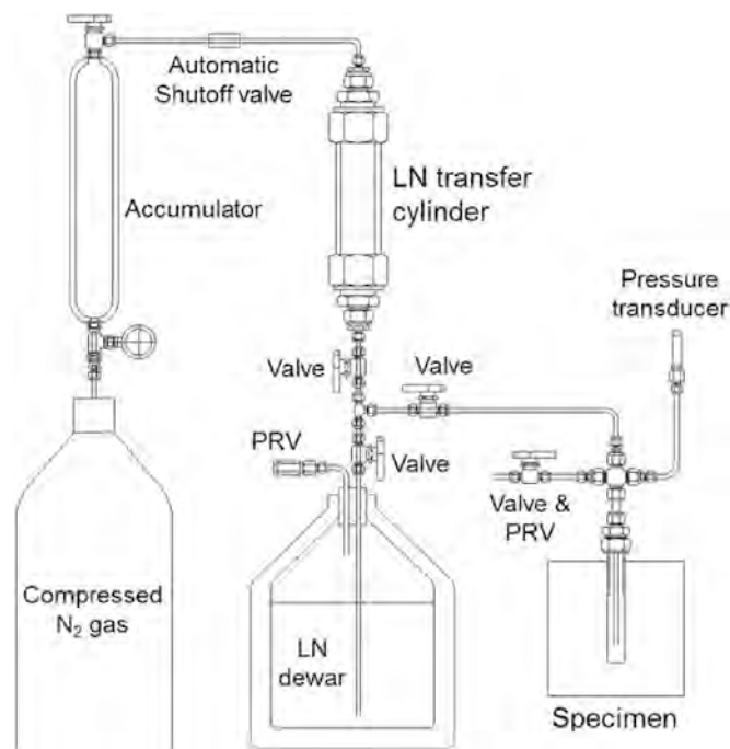
Fig. 3. Schematic of lab cryogenic stimulation setup for higher-pressure LN flow. LN is temporarily stored in the transfer cylinder from the dewar, and compressed nitrogen gas is used to push LN to specimen boreholes.
