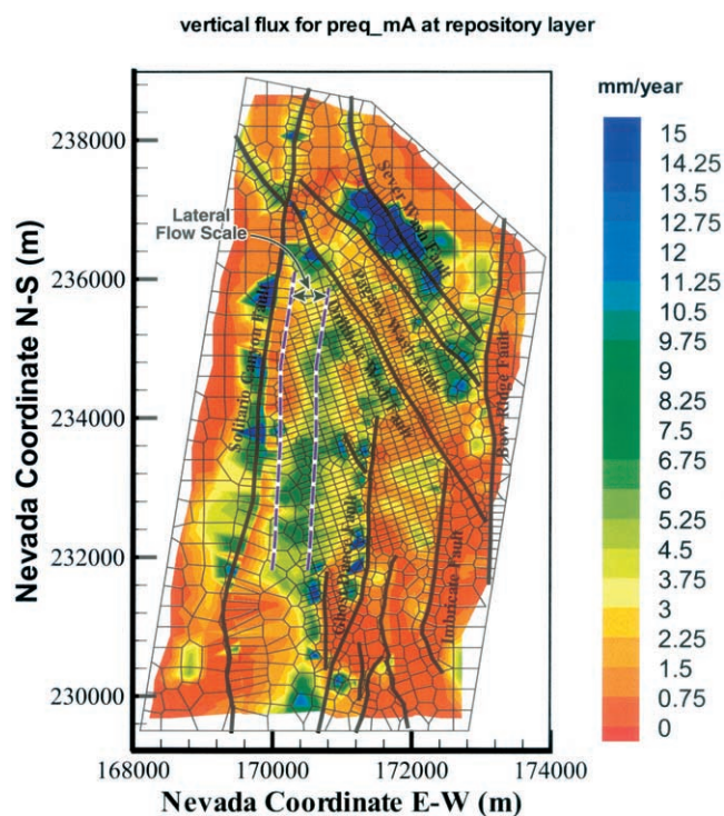
Fig. 9. Simulated percolation fluxes at the proposed repository horizon for base case present-day, mean infiltration using the results of simulation req_mA.
