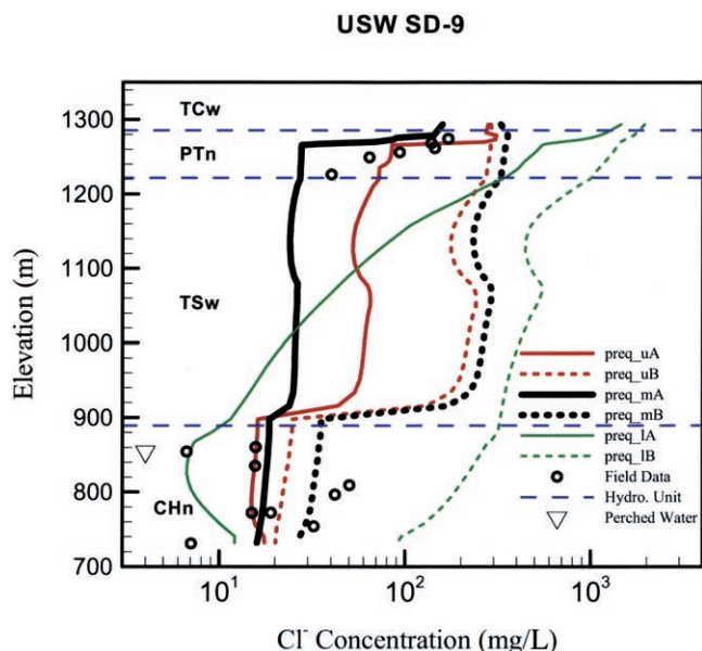
Fig. 8. Comparison between measured and simulated \text{Cl}^- concentration profiles at Borehole SD-9 for present infiltration with mean, upper, and lower bounds with six flow fields (req_uA, req_mA, req_lA, req_uB, req_mB, and req_lB).
